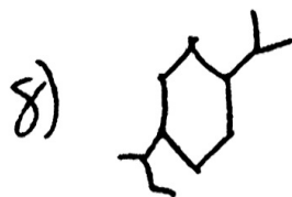
1-sec-butyl-4-isopropylcyclohexane
