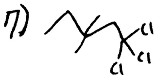
1,1,1-trichloro-2,2-dimethylpentane
